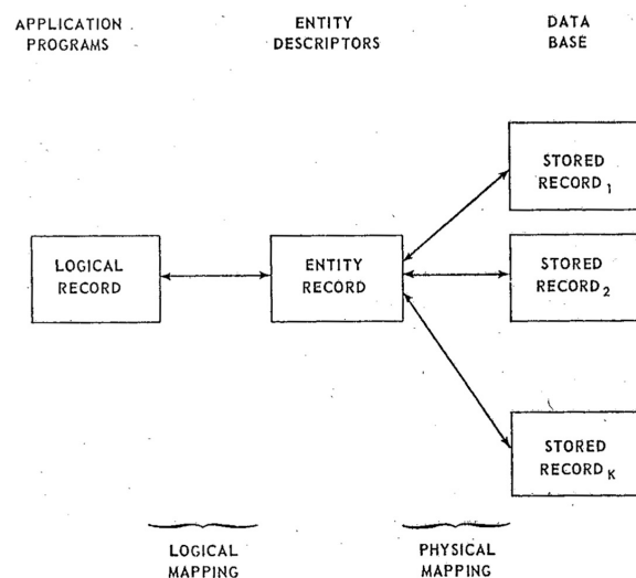
Abb. 13: GUIDE-SHARE-Datenbankarchitektur (Joint GUIDE-SHARE Database Requirements Group 1970: 3.5)
