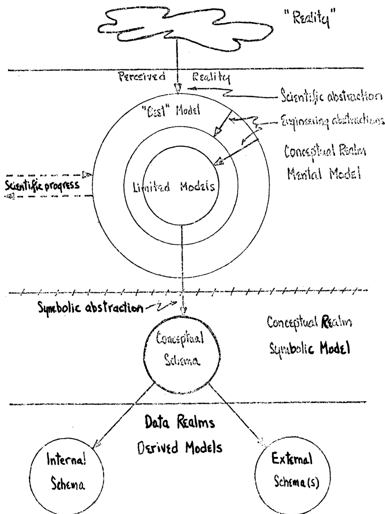
Abb. 17: Not just Reality - Data (Study Group on Data Base Management Systems 1975: VIII-32)
