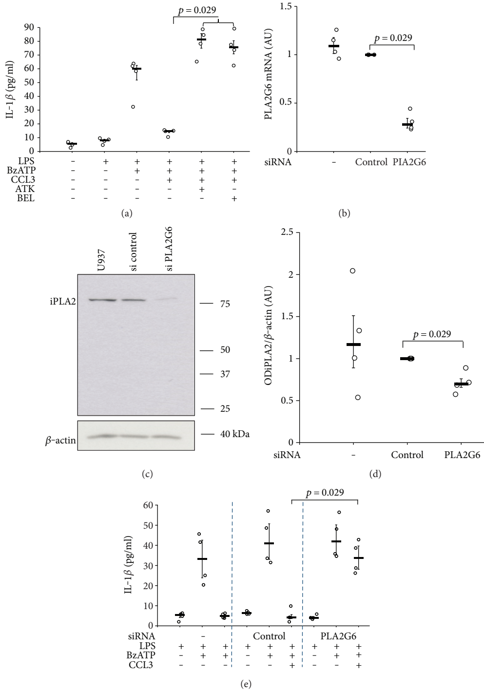
FIGURE 6: CCL3 signaling involves calcium-independent phospholipase A2 (iPLA2). Human monocytic U937 cells were primed with LPS (1 μg/ml, 5 h) and activated 2'(3')-O-(4-Benzoylbenzoyl)adenosine-5'-triphosphate (BzATP; 100 μM, 30 min). The release of IL-1β to the cell culture supernatant was measured by ELISA. (a) CCL3 (10 ng/ml) inhibited the release of IL-1β in response to BzATP. The general PLA2 inhibitor arachidonyl trifluoromethyl ketone (ATK) and the specific iPLA2 inhibitor bromoenol lactone (BEL) reversed CCL3-dependent inhibition. (b–e) Expression of iPLA2 by U937 cells was silenced by siRNA ( PLA2G6 ); scrambled siRNA served as control. Silencing of PLA2G6 expression was efficient as revealed by real-time RT-PCR (b) and by Western blotting (c, d). Data in (b) and (d) are given as arbitrary units. (c, d) In Western blotting experiments, β-actin served as a loading control, the optical density (OD) of the immunopositive bands was measured, and the ratio of the OD of iPLA2 and β-actin was formed. (b, d) Values obtained for cells treated with siRNA targeting CCR1 were statistically compared to those transfected with control siRNA. (e) After treatment with siRNA targeting PLA2G6 expression, the inhibitory effect of CCL3 on IL-1β release was blunted. In untreated control cells and upon transfection of control siRNA, CCL3 was effective. Data are presented as individual data points, bars indicate median, and whiskers percentiles are 25 and 75, n = 4, each.
