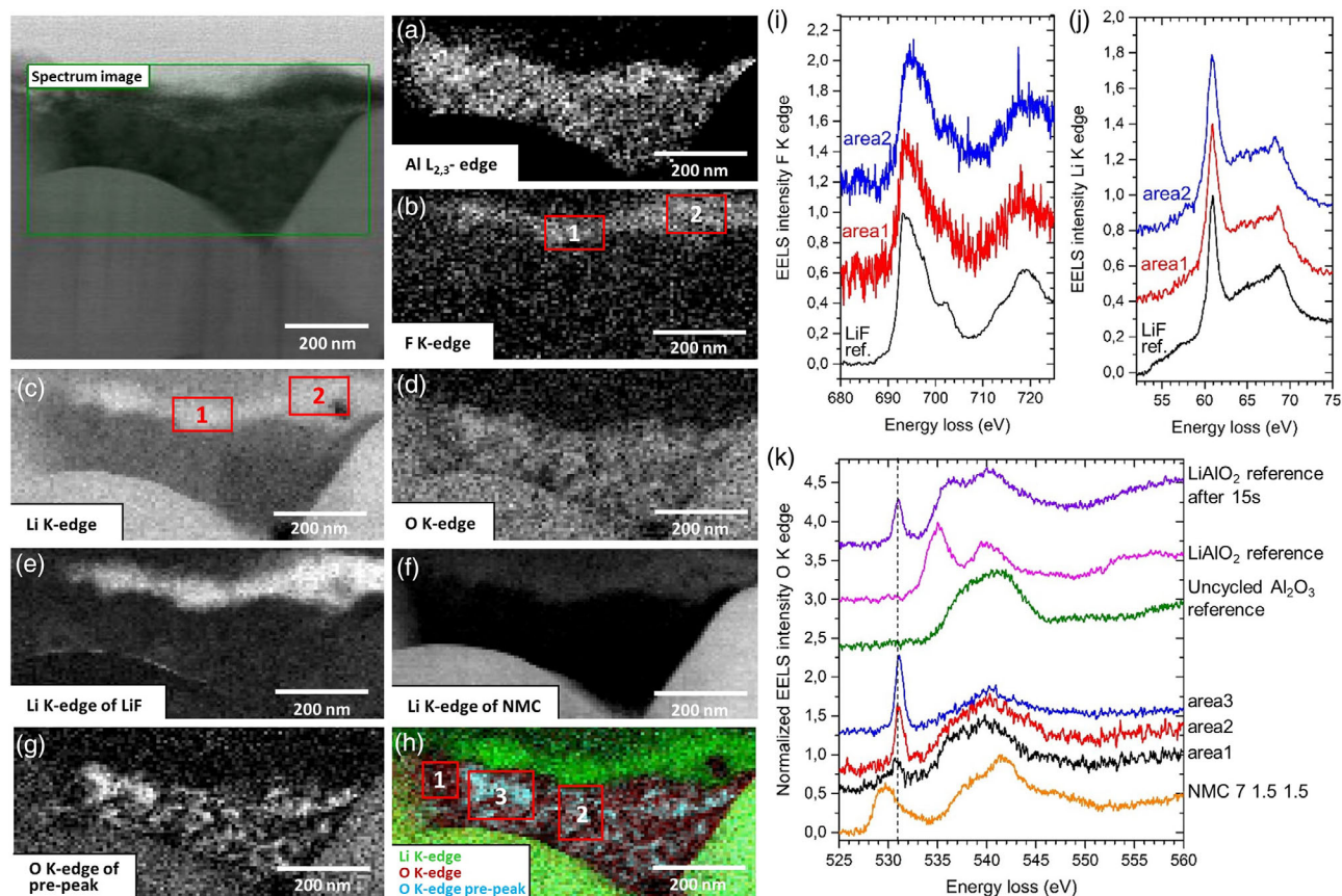
Figure 12. STEM-EELS analysis and spectra of selected areas of a cross section of cycled NMC701515 coated with 1 wt% fumed \text{Al}_2\text{O}_3 . Compositional spectrum images corresponding to the Al L_{2,3} -edge, F, Li, and O K-edges are, respectively, shown on panels a)–d). e), f) The MLLS fitting of the Li K-edge region using fine structures corresponding to LiF and NMC701515. g) The distribution of the prepeak to the O K-edge integrated between 528 and 532 eV (it is important to note that contrast in the NMC701515 is due to the presence of spectral weight at the O K-edge of NMC701515 in this same energy range as visible in panel (k)). h) A false color image of the Li K-edge (green), O K-edge (red), and prepeak of the O K-edge (blue). i, j) The experimental ELNES spectra of the F and Li K-edges, respectively, in areas 1 and 2 of panels (b) and (c) compared with a reference spectra taken on a commercial LiF powder, confirming the presence of a LiF layer at the surface of the coating. k) Spectra of the O K-edge taken in areas 1, 2, and 3 of panel (h) compared with uncycled \text{Al}_2\text{O}_3 and \text{LiAlO}_2 reference spectra.
