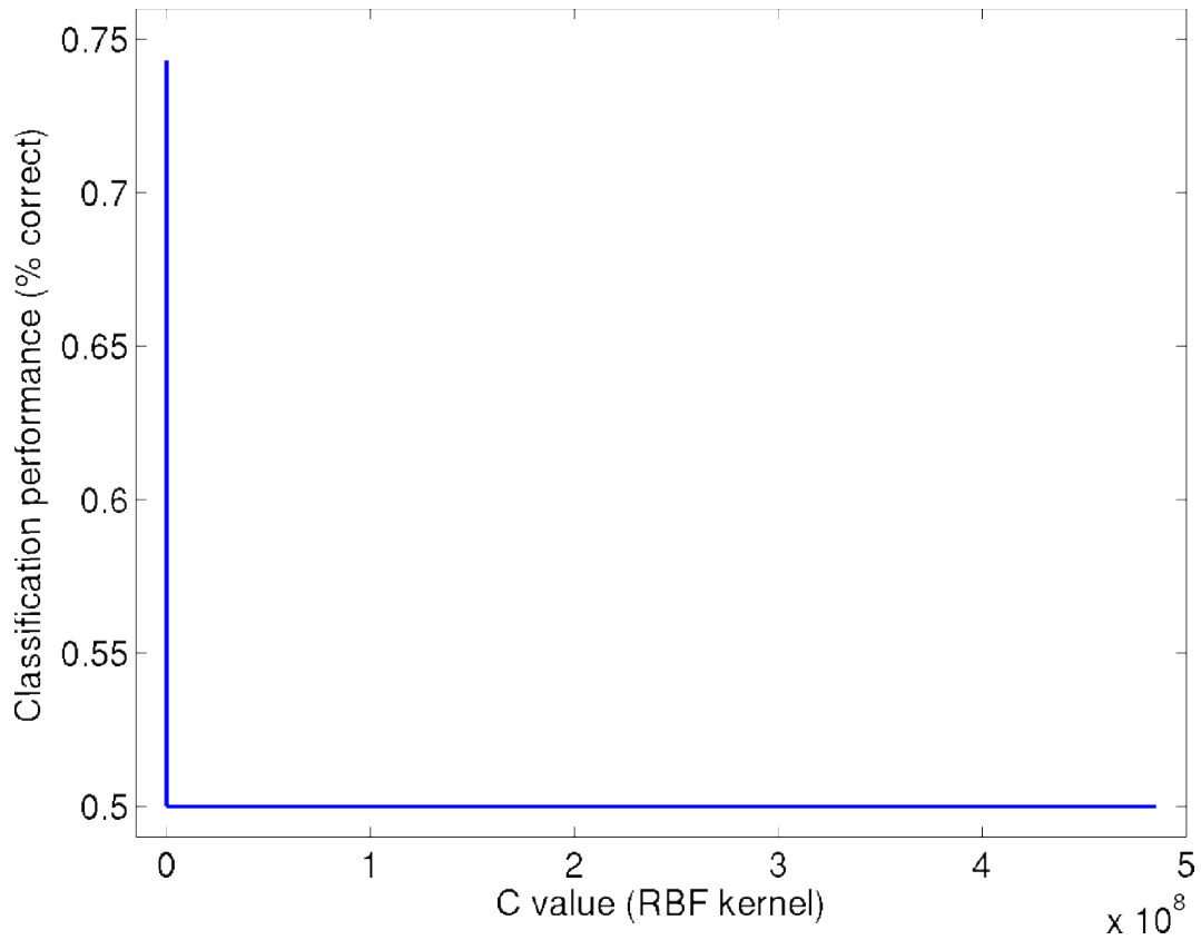
Illustration 94: Exemplary result of a C-value search, first stage. A significant maximum close to zero can be seen
