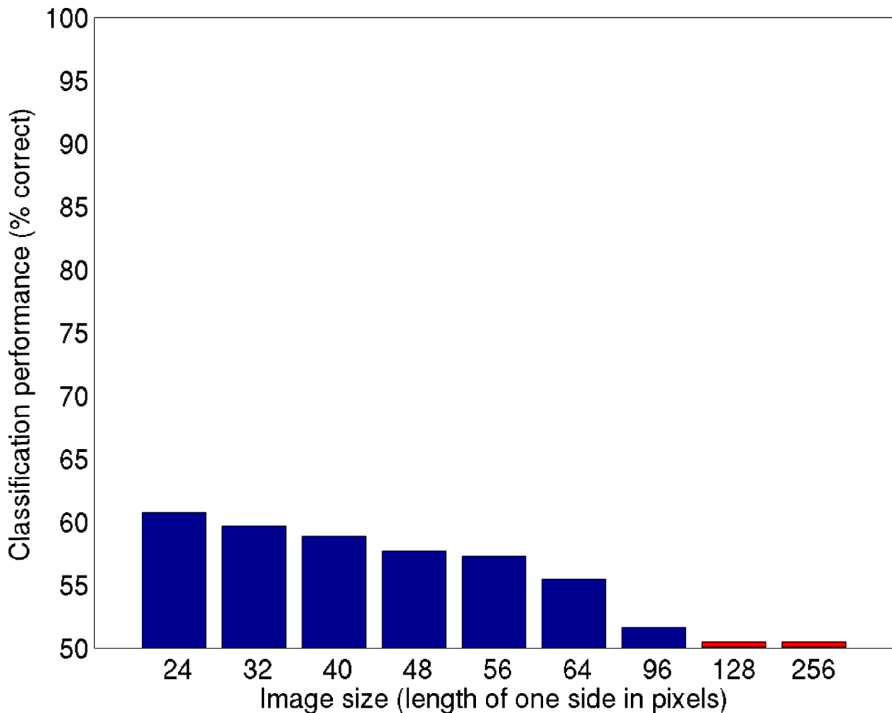
Illustration 32: Classification performance on pixel intensity values of various image sizes
