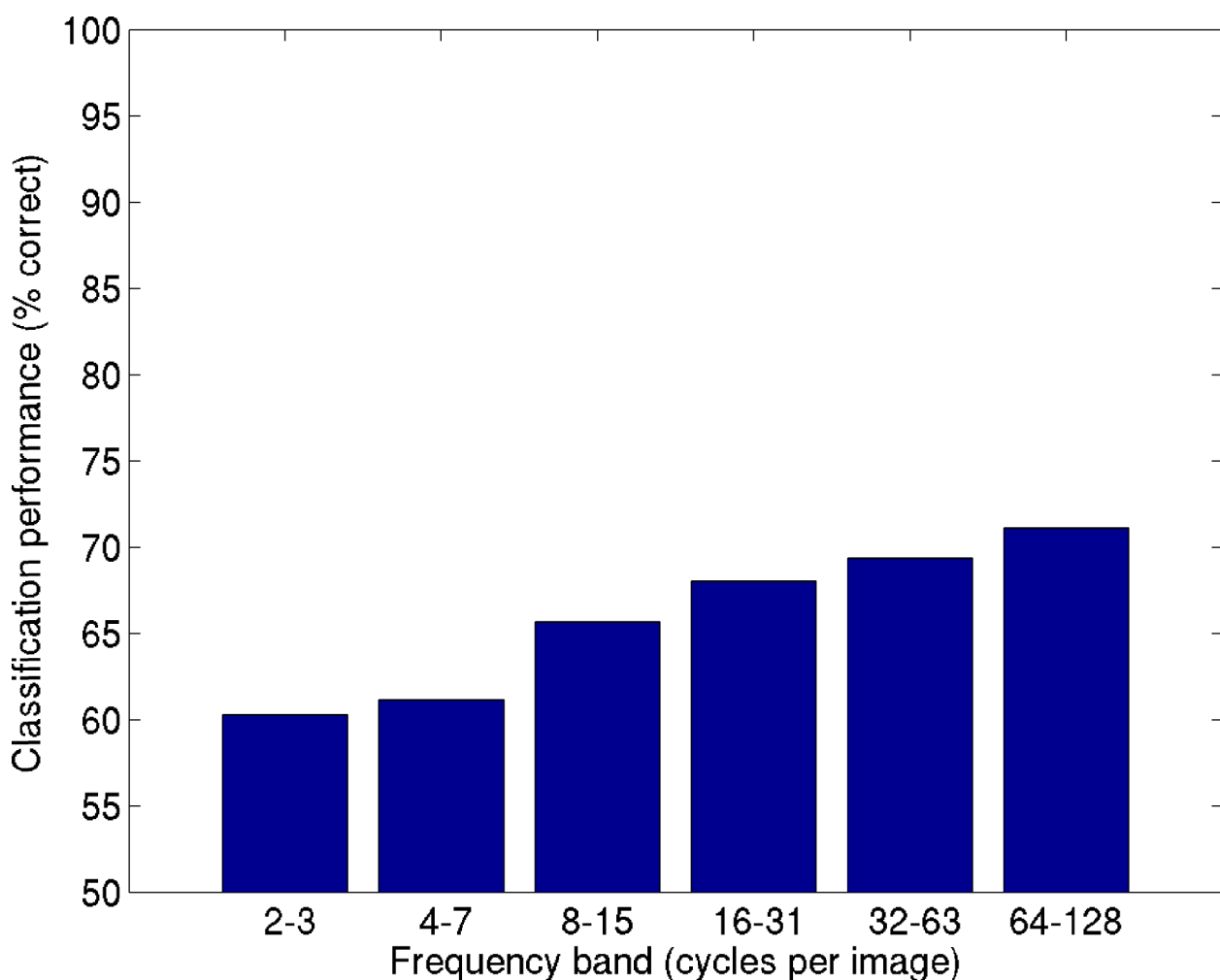
Illustration 44: Classification performance on frequency bands
