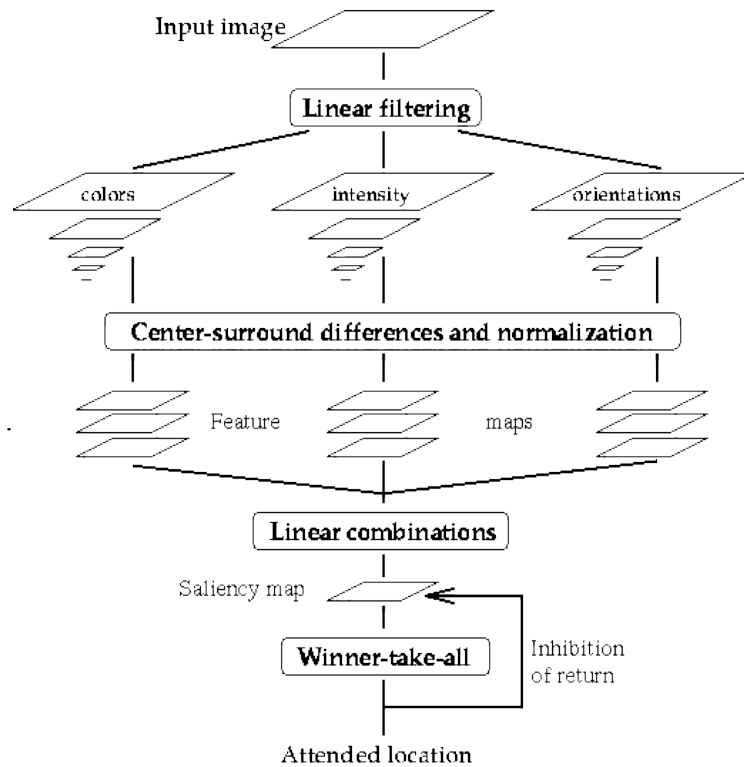
Illustration 3: The model of saliency as proposed by Itti, Koch and Niebur [Itti Koch Niebur 1998]
