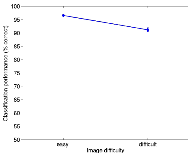
Illustration 64: Classification performance
