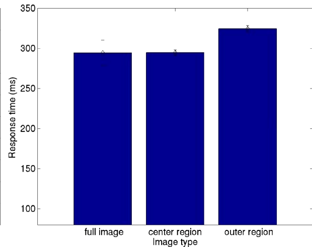
Illustration 92: Experiment 4: Response times
