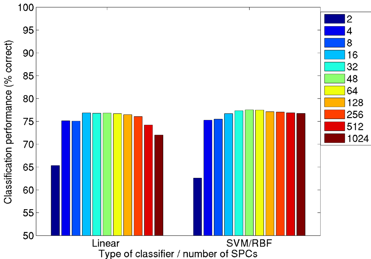
Illustration 38: Classification performance on SPCs of size 256 pixels, linear vs. support vector classifier
