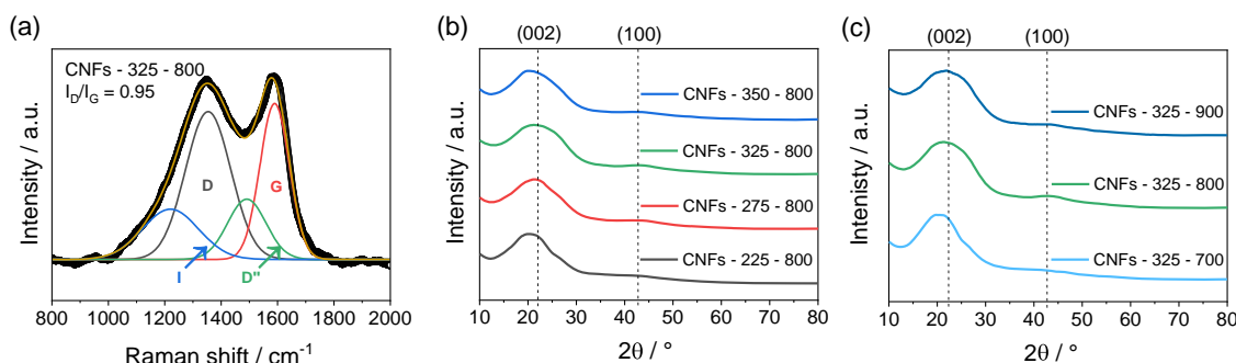
Figure 7. a) Raman spectrum of the CNF—325—800 sample. b) XRD patterns of CNFs samples prepared with varying T_s from 225 °C up to 350 °C and a constant T_c at 800 °C. c) XRD patterns of CNFs stabilized at 325 °C with varying T_c from 700 °C up to 900 °C. These structures correspond to JCPDS 00-056-0159.
