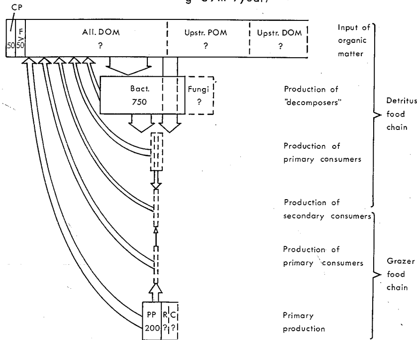
Fig. 2. Hypothetical trophic structure in the middle reach of the Breitenbach. Grazer and detritus food chains are separated, as in CUMMINS et al. (1966). For explanations see Fig. 1.
