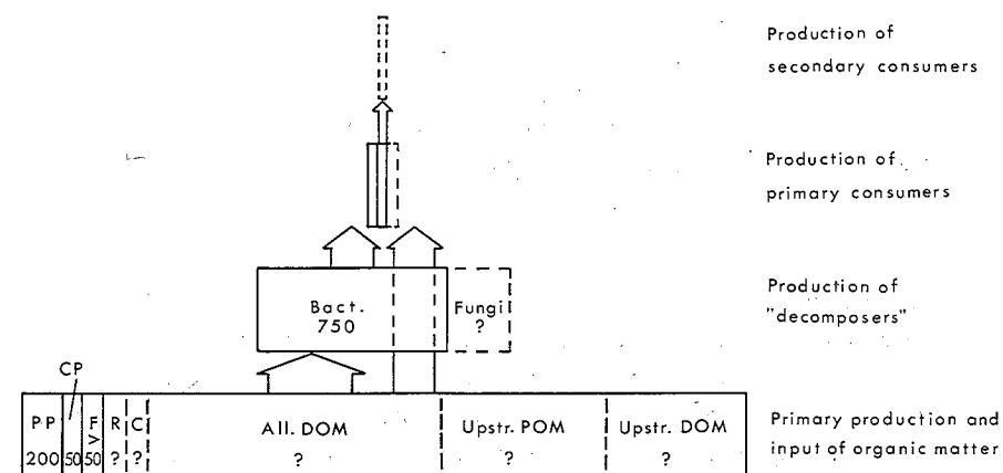
Fig. 1. Hypothetical production pyramid for the middle reach of the Breitenbach. The solid lines enclose compartments for which at least estimated values are known; no values are known for compartments which are limited by dashed lines. In this figure the detritus and grazer food chains are combined to emphasize the quantitative importance of bacteria. PP — primary production (excl. release of dissolved organic matter), CP — coarse particulate allochthonous organic matter, F — fine particulate allochthonous organic matter, R — release of dissolved organic matter by primary producers, C — chemoautotrophic production, All. DOM — allochthonous dissolved organic matter, Upstr. POM — particulate organic matter from upstream, Upstr. DOM — dissolved organic matter from upstream. For the origin of data see Table 3.
