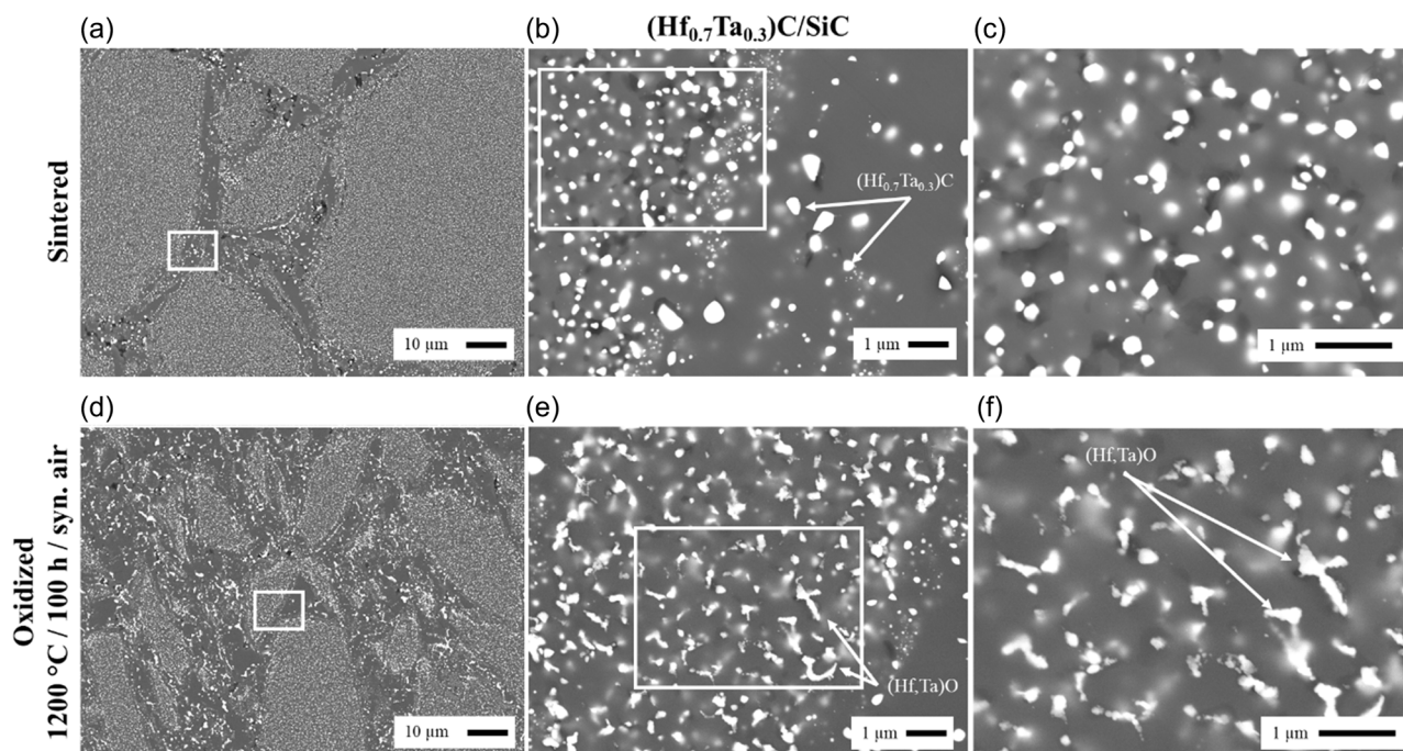
Figure 7. BSE images of (\text{Hf}_{0.7}\text{Ta}_{0.3})\text{C}/\text{SiC} in the sintered state a–c) and after exposure at 1200 °C for 100 h in dry synthetic air d–f).
