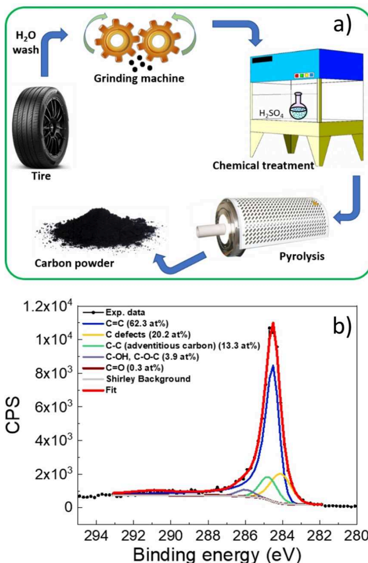
Figure 1. (a) Schematic representation of the process applied for the preparation of the carbon-based material employed as CE component for C-PSCs in the present work, starting from waste tires. (b) XPS spectrum of the C 1s region of the obtained carbon material.
