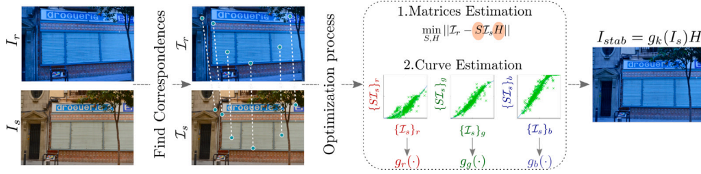
Fig. 2. Flowchart of the proposed method. Given two images, a reference I_r and a source I_s , we first compute a set of correspondences between them, and we denote the pixel values at those correspondences as I_r and I_s , respectively. Within the optimization process, we estimate the two matrices S and H from Eq. (8), and then we estimate the curve g(\cdot) for each color channel. The final color stabilized image is then computed as g_k(I_s)H , k = \{R, G, B\} .
