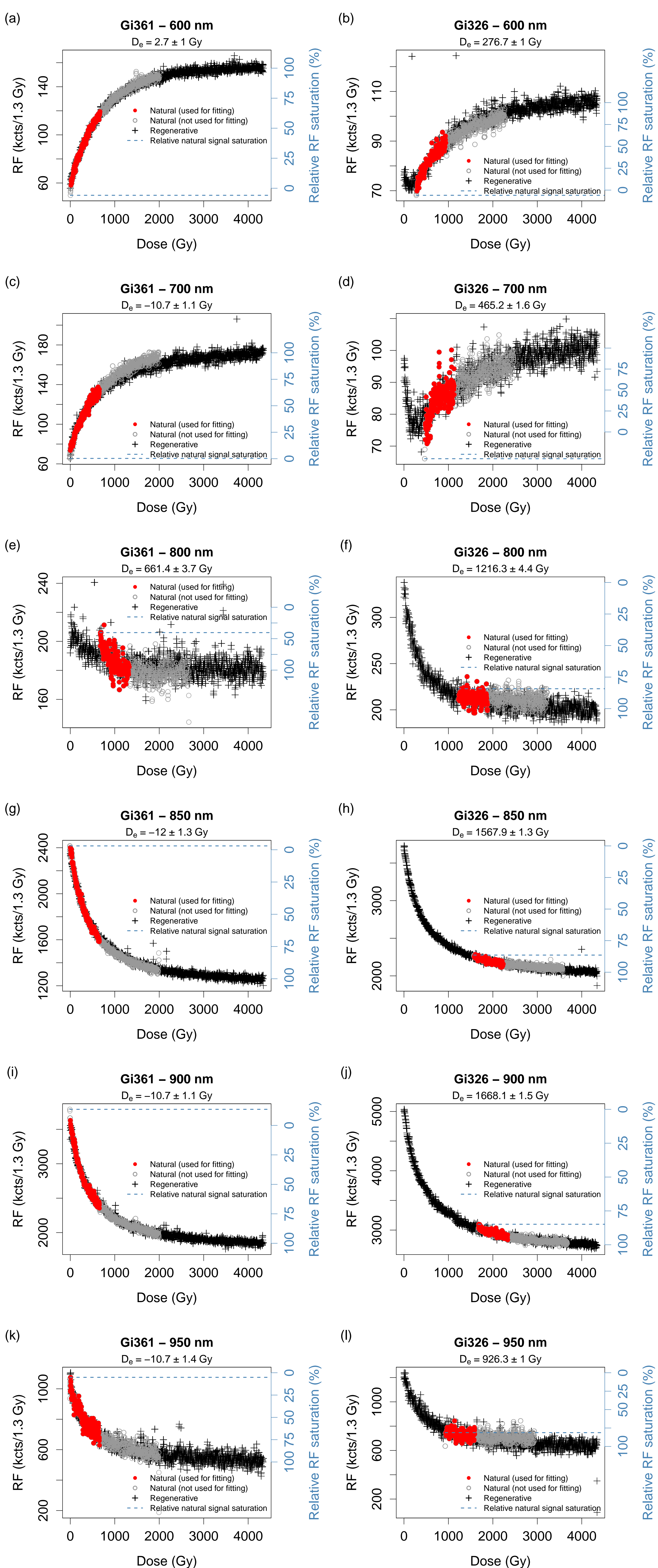
Figure S1: Examples of spectroscopic RF D_e estimation at six wavelengths of one aliquot of Gi361 (left-hand column) and Gi326 (right-hand column) at around (a, b) 600 nm, (c, d) 700 nm, (e, f) 800 nm, (g, h) 850 nm, (i, j) 900 nm and (k, l) 950 nm.
