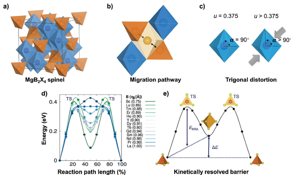
Figure 4. a) The \text{MgB}_2\text{X}_4 spinel crystal structure is shown on the left with the B-cation shown in blue and the Mg-cation in orange. b) The \text{Mg}^{2+} migration follows an interstitial mechanism. \text{Mg}^{2+} is tetrahedrally coordinated at the initial and final sites (orange) and migrates through empty octahedral (light orange) sites following a tet-oct-tet migration path. The transition state (TS) of the migration process is the triangular face shared by initial tetrahedral and intermediate octahedral sites. c) The trigonal distortion of octahedron specified by anion parameter u and the angle \alpha . d) The energy along the migration path for \text{MgB}_2\text{Se}_4 spinel compounds determined by NEB. e) Schematic of the energy profile of the \text{Mg}^{2+} migration. The kinetically resolved barrier E_{KRA} and the difference in energy between tetrahedral and octahedral sites referred as site preference energy \Delta E are indicated by arrows.
