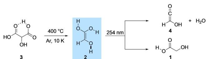
Scheme 1. 1,1,2-Ethentriol ( 2 ) generated from tartronic acid ( 3 ) through pyrolysis and trapping in an argon matrix as well as the subsequent photorearrangement to glycolic acid ( 1 ) and ketene ( 4 ).
