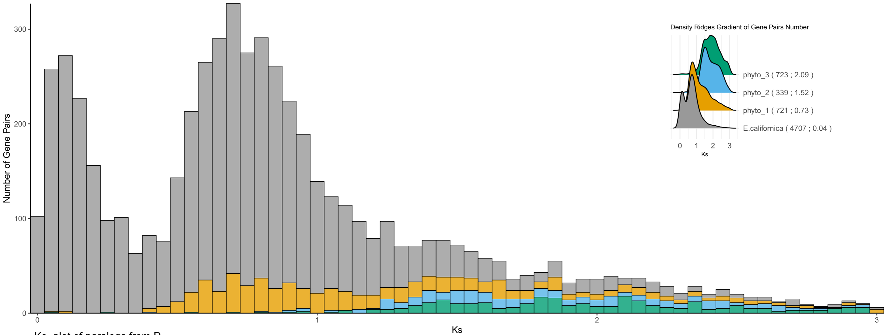
Ks-plot of paralogs from P
