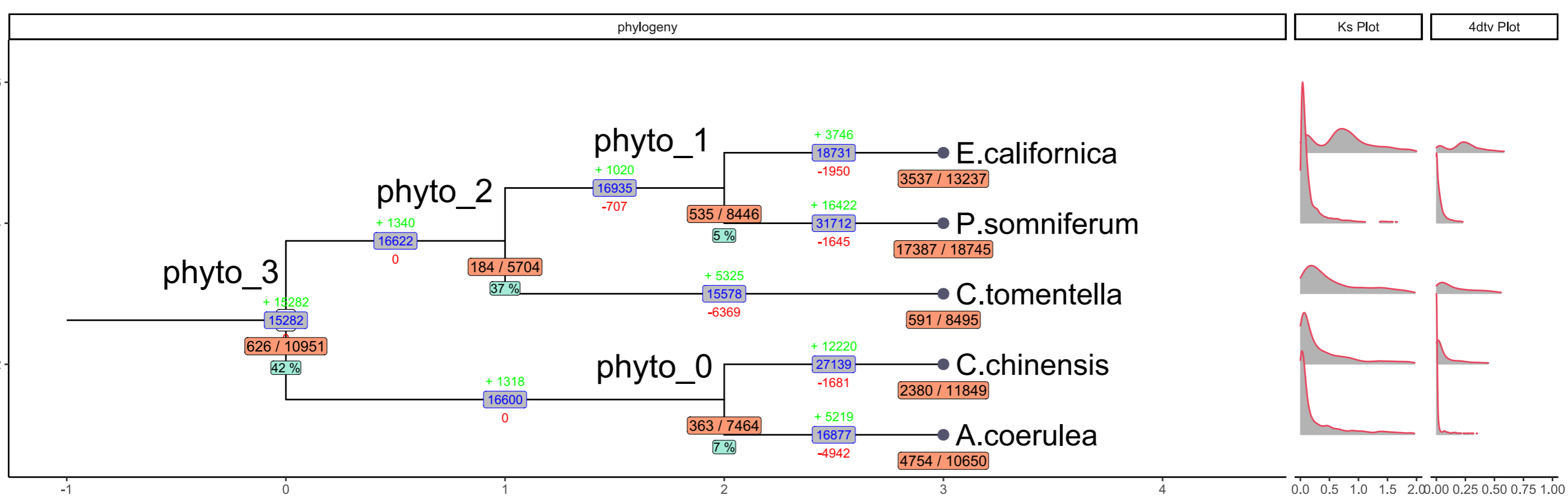
Ks-plot of paralogs from C
