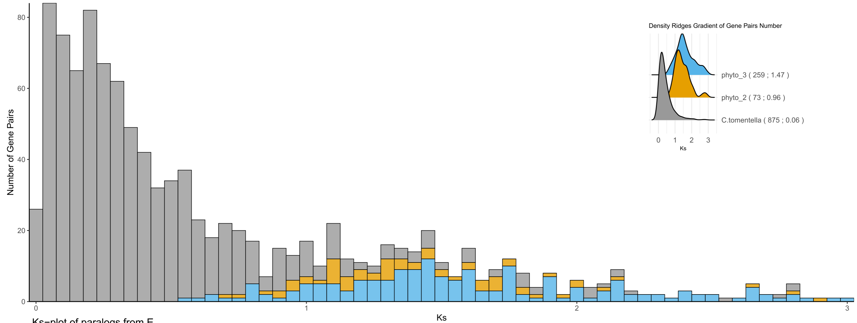
Ks-plot of paralogs from E
