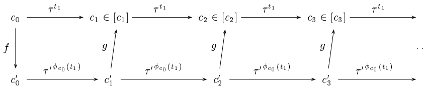
Figure 2: Illustration of a uniform simulation.
