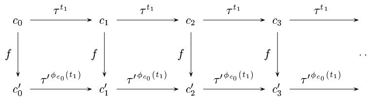
Figure 3: Illustration of a strong uniform simulation.
