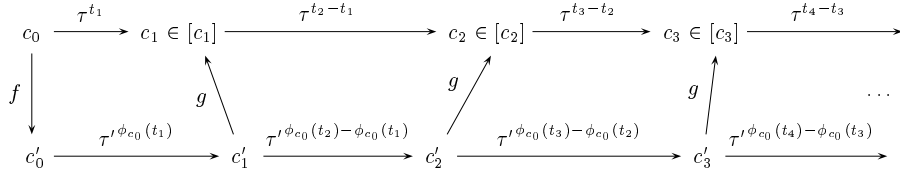
Figure 1: Illustration of a simulation.
