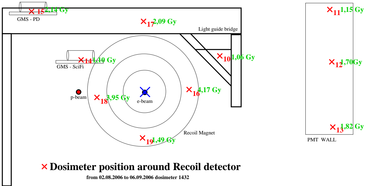
Figure 5.31: RPL dosimeter position surrounding the Recoil Detector and dose collected from 02.08.2006 to 06.09.2006.
