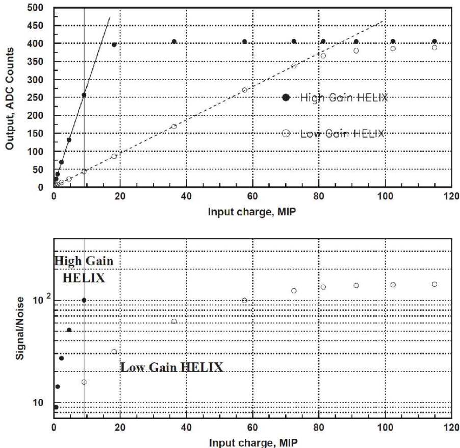
Figure 4.8: Measured response of the readout electronics against the charge injected at the input. Illustration of the increase of the dynamic range of the silicon detector. Every Silicon strip was connected with two readout channels, one high gain channel and one low gain channel through a capacitor.
