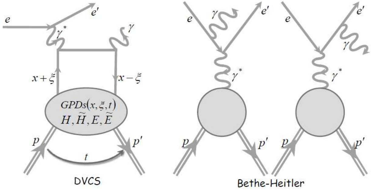
Figure 3.5: Feynman Graphs for DVCS (left panel) and Bethe-Heitler process (right panel). Both processes lead to the same final state.
