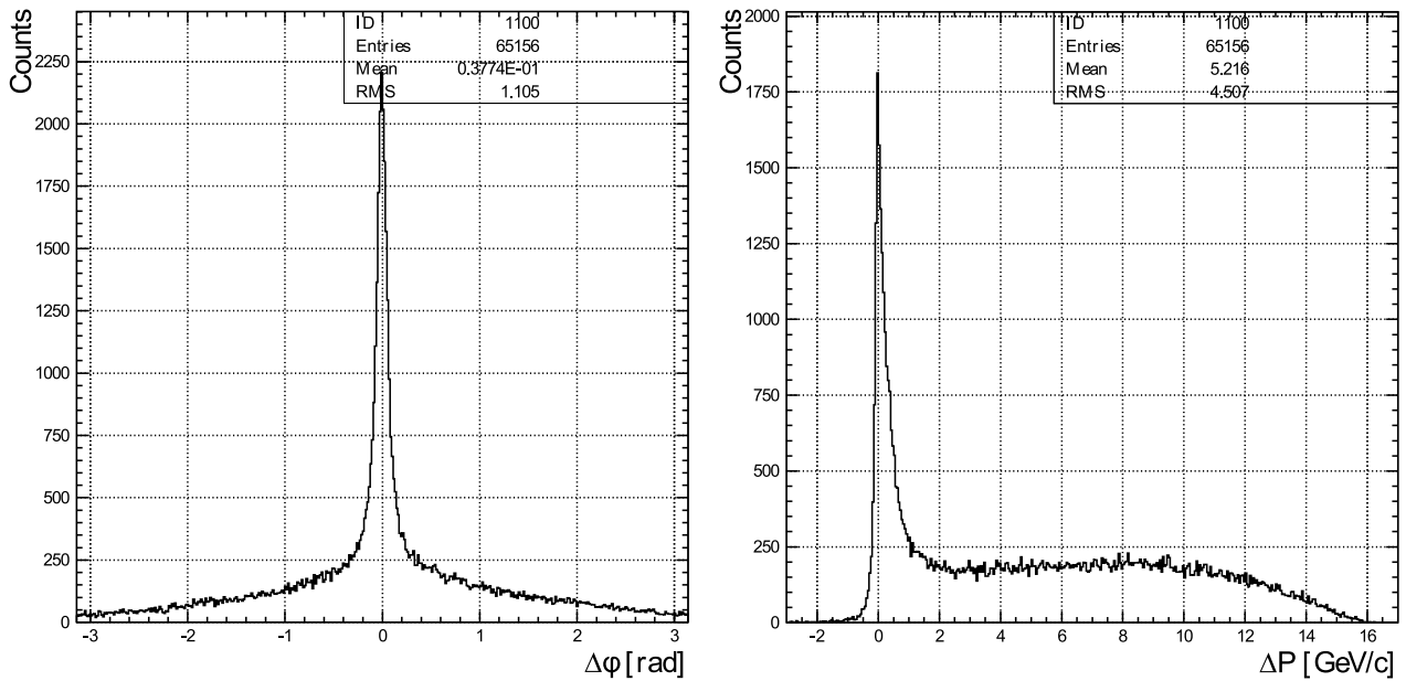
Figure 7.5: \Delta p and \Delta\phi distribution of the recoil protons. These two variables were used to reduce the background, the cut were set around the peak as 0.1\text{ rad} for the difference between the azimuthal angle reconstructed from the observed and as 1.00\text{ GeV}/c for the difference between the momenta.
